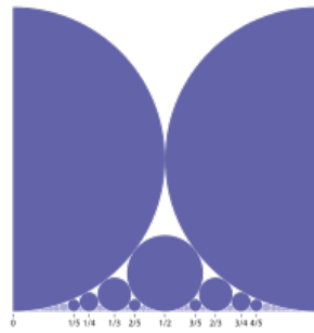
Ford circles
