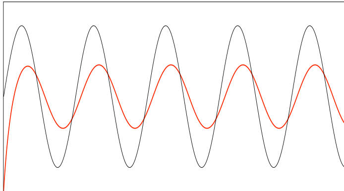
Response (red) to an alternate tension (black).
