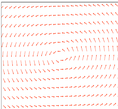
Magnetic field in the plane.
