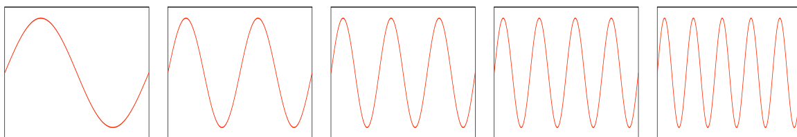
Wave functions of the first 5 energy levels.
