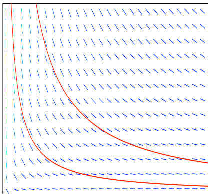
Directions field and two homothetic solutions of the homogeneous equation \dot{y} = -y/x .
