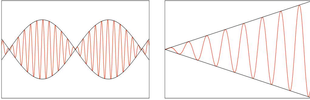
Beats and resonance.
