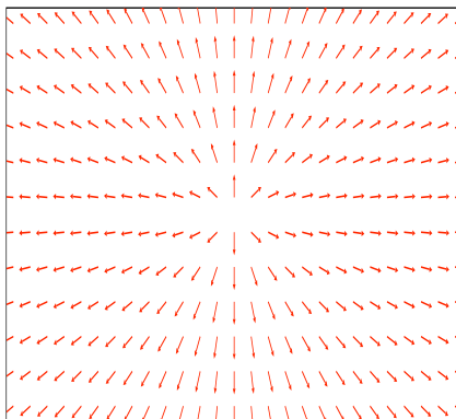
Electric field generated by a charge at the origin.
